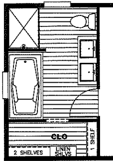
BATH OPT. 2 76' & 80' OPTS ONLY
