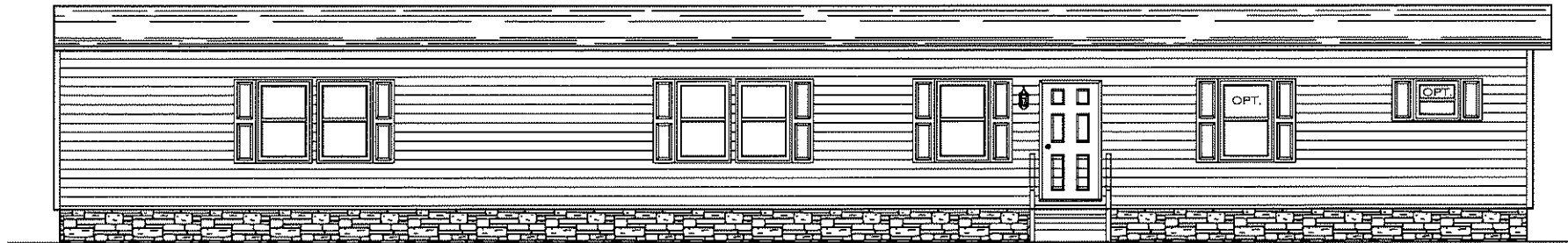
FRONT ELEVATION
