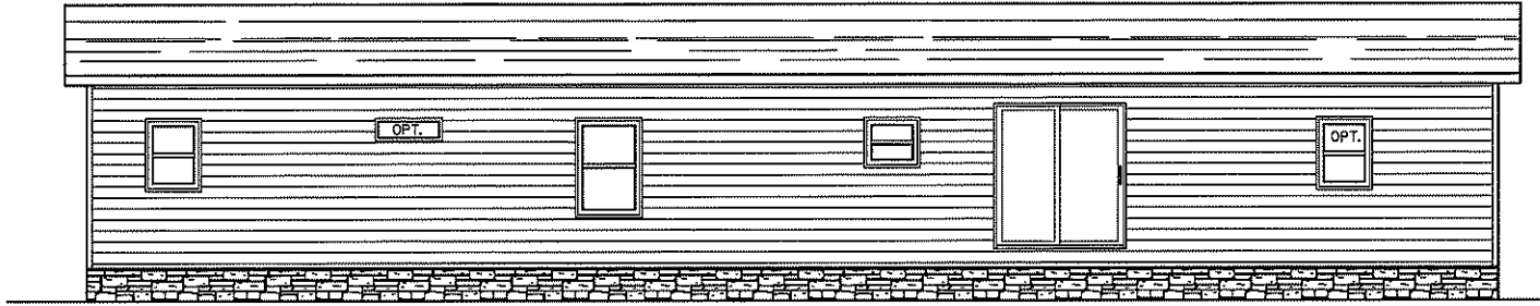
REAR ELEVATION
