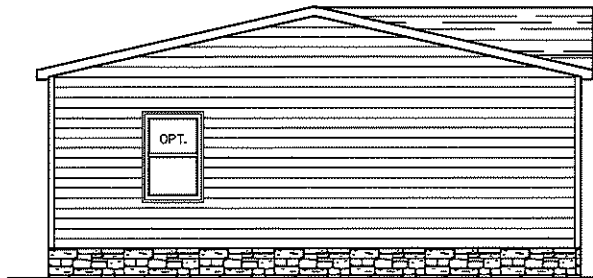
LEFT ELEVATION
