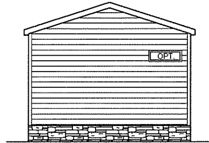
LEFT ELEVATION
